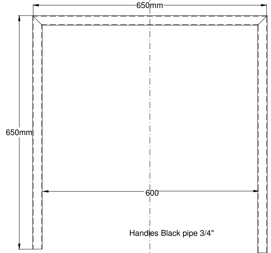
Donkey Scoop Drawbar and Handles D2
